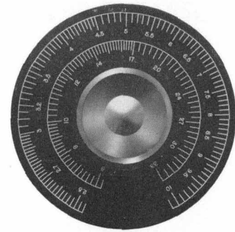
Fig. 6. High resolution frequency dial on Model 200T has effective scale length of about 65 inches. Scales are laid out to facilitate RDB telemetering work.
