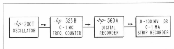
Equipment arrangement used to automatically record stability characteristics of hp -Model 200T.
