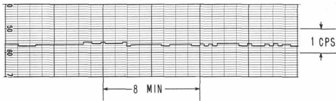
Fig. 3. Typical stability characteristic of hp Model 200T operating at 10 kc after warmup. Note that major division equals only 1 cps of change.
